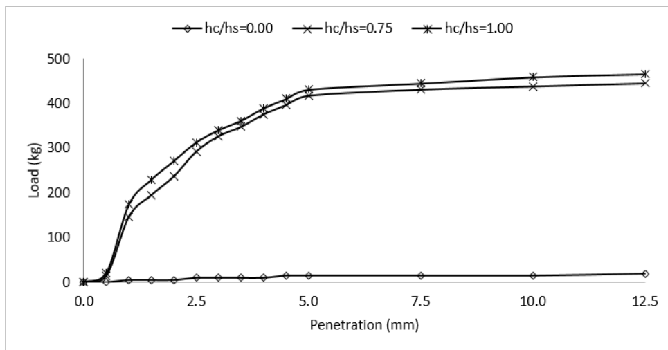
Fig. 2 CBR of cushion-soil system with 8% lime in the cushion after soaking
